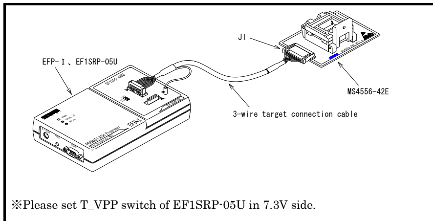
Fig.2.1 Connection with EF1TGCB-A (3-Wire Target Connection Cable)
