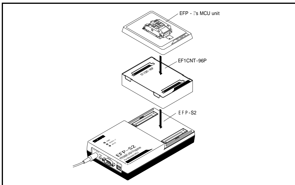
Fig.2.1: MCU Unit Mounting Method
