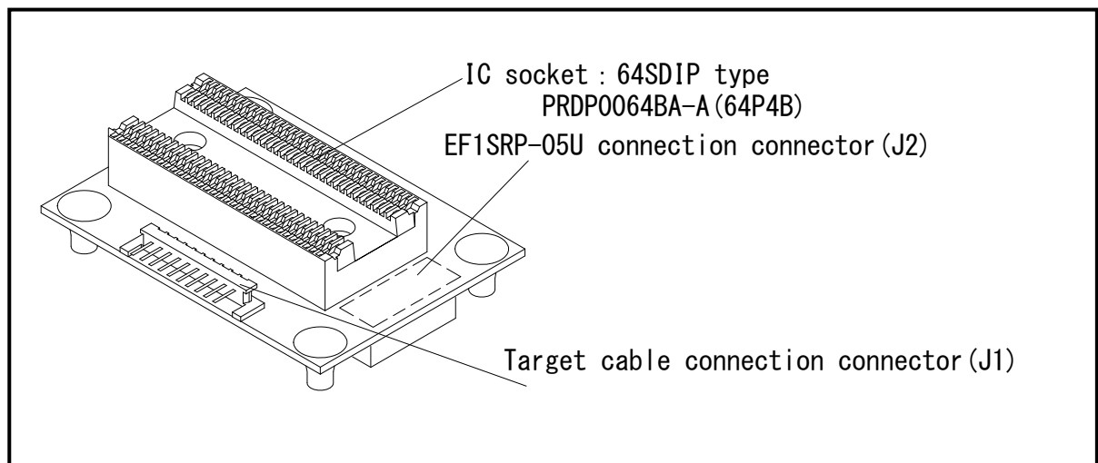
Fig 1.1 MS3803-64S External Figure
