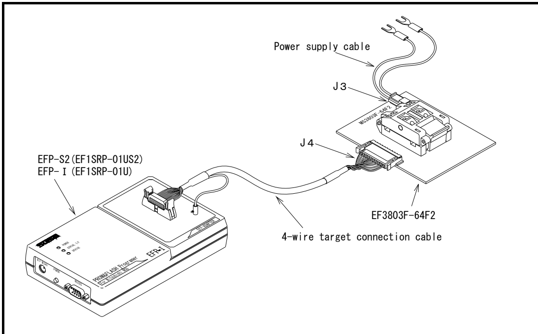
Fig 2.1 Connection with MS3803F-64F2
