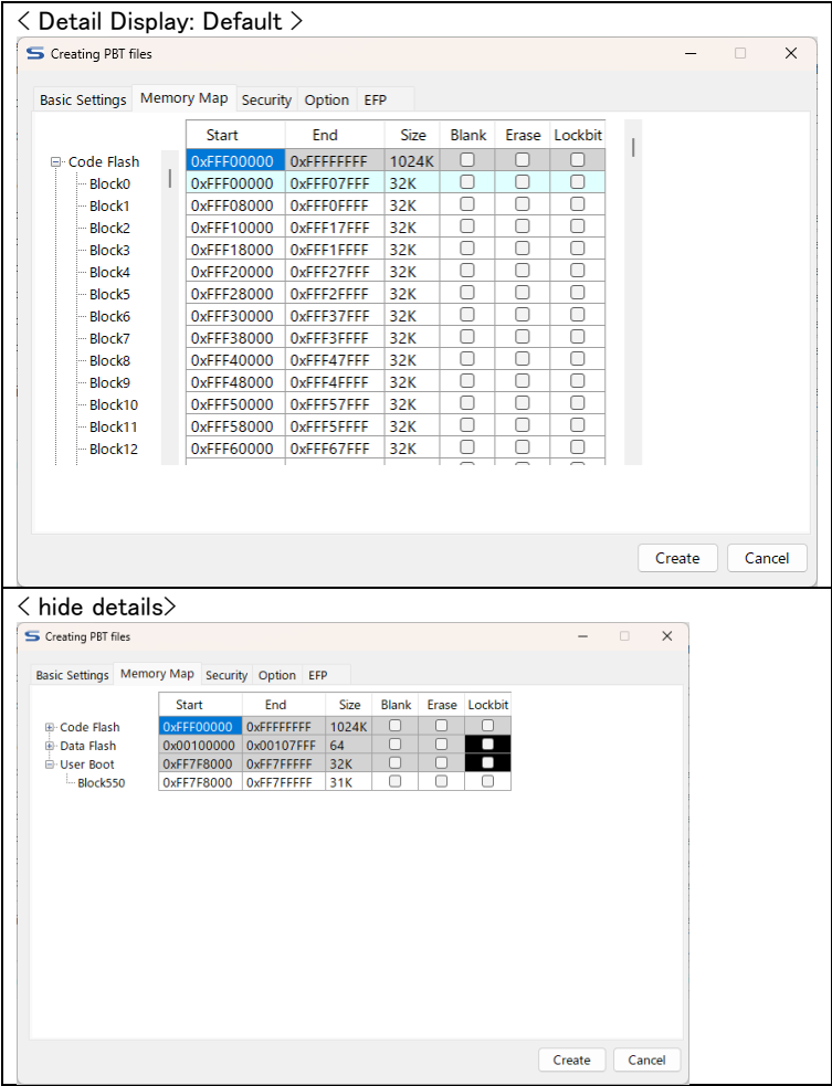
Figure 4.10 Memory Map Tab
