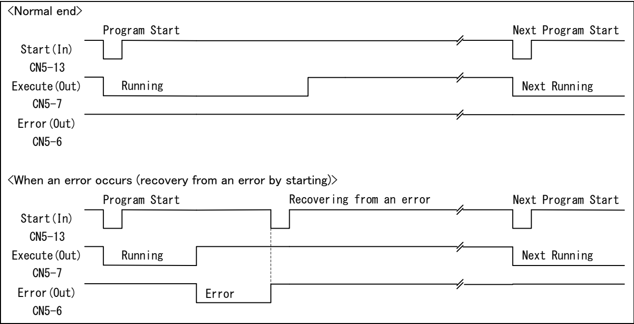
Figure 1.6 External Control Signal Sequences
