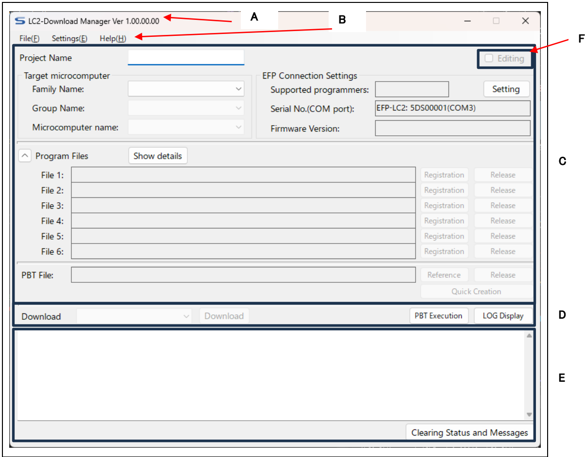
Figure 4.1 Main screen immediately after installation
