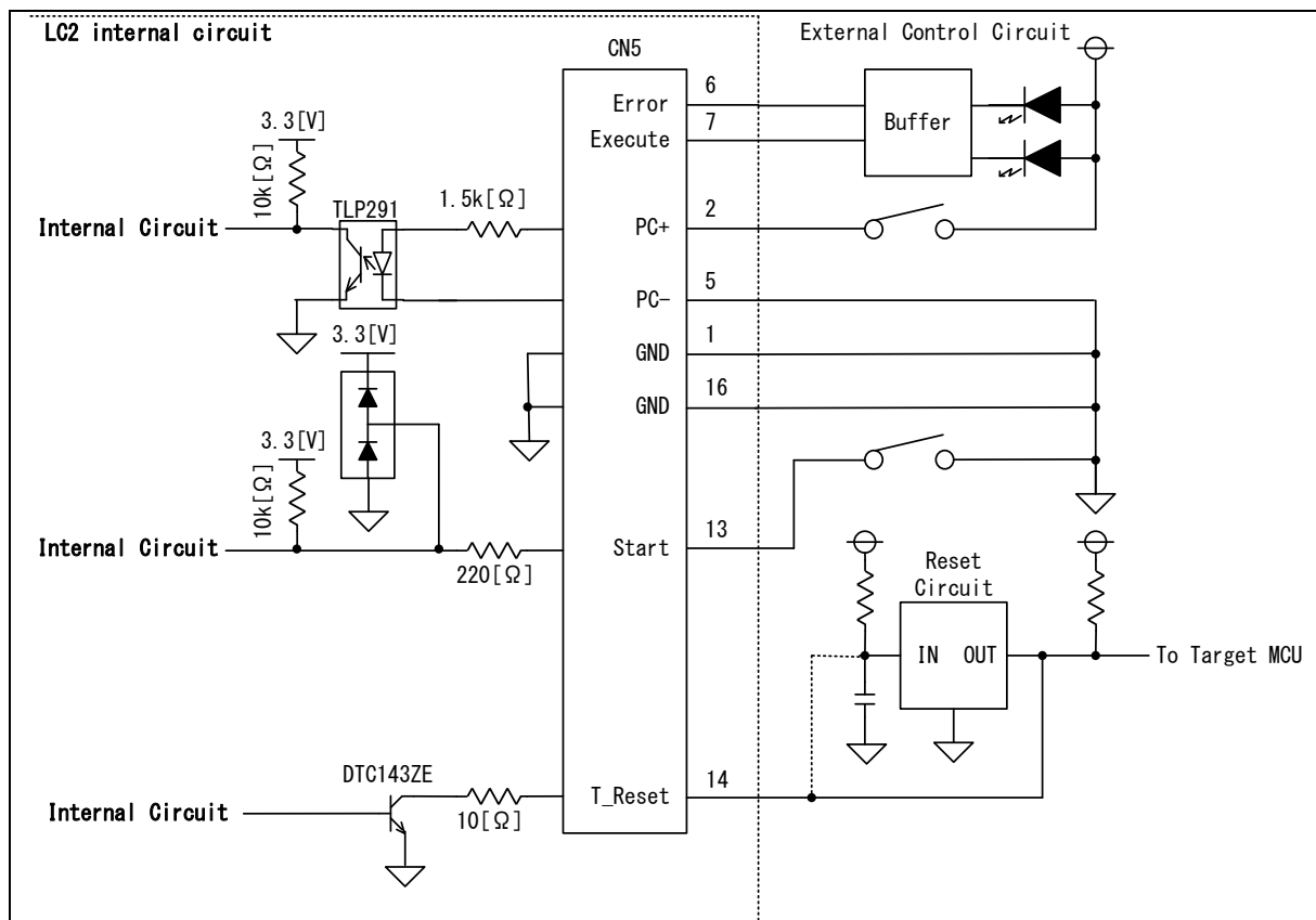
Figure 1.5 Example of external control signal connection
