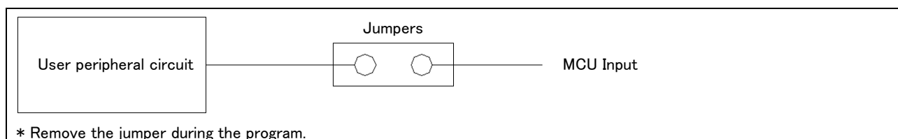
Figure 1.3 Example of collision prevention circuit using jumpers
