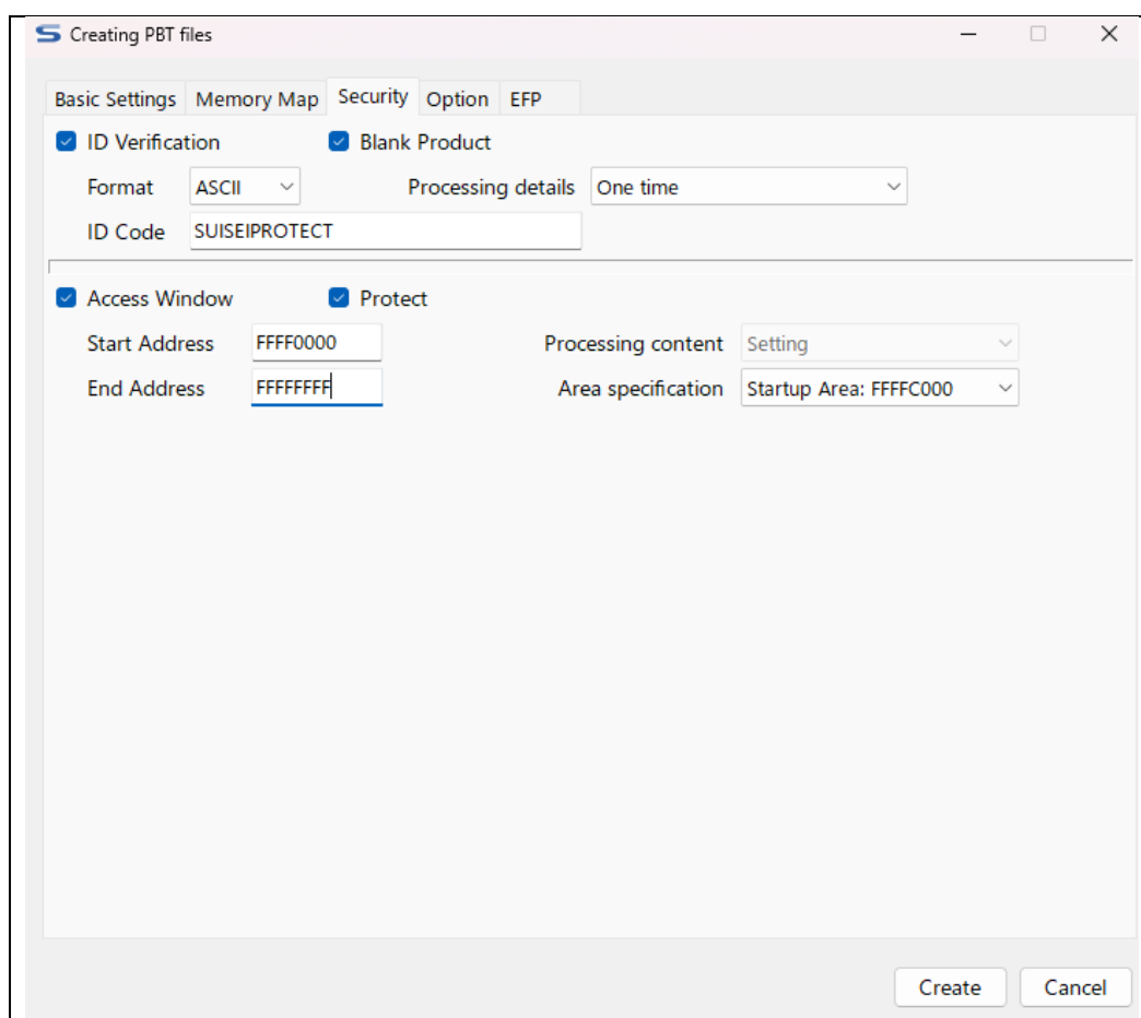
Figure 2.3 Security Tab
