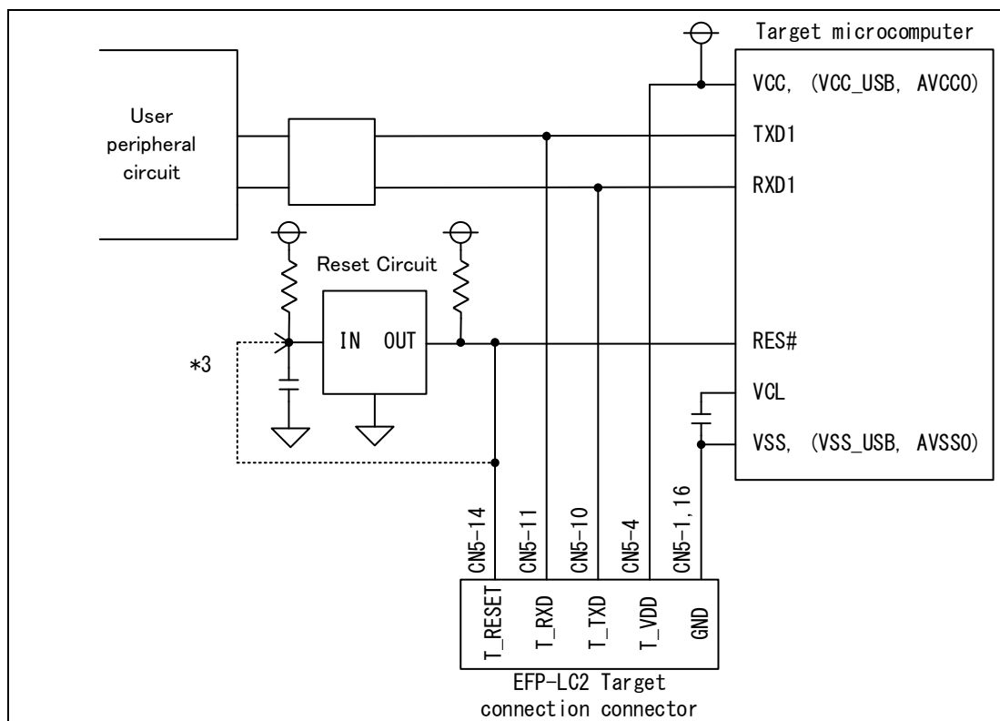
Figure 1.2 Target System Recommended Schematic
