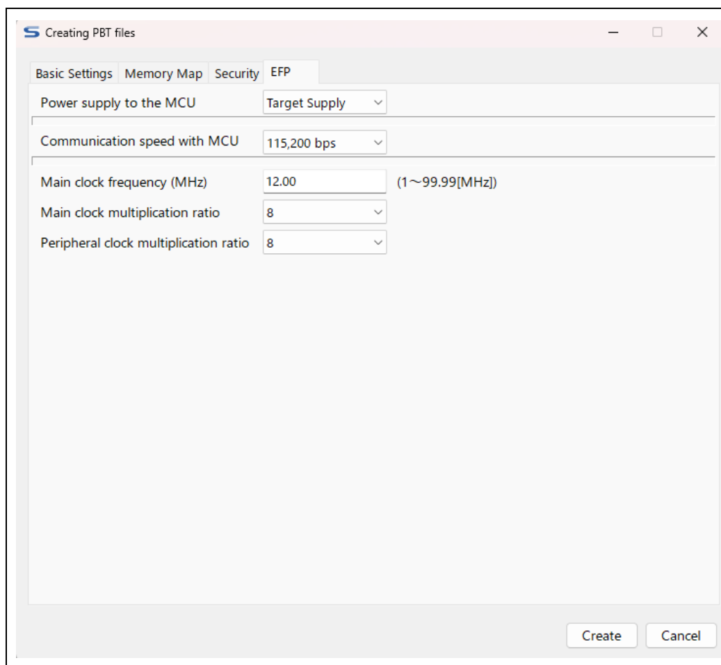
Figure 2.5 EFP Tab
