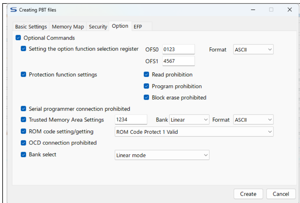
Figure 2.4 Option Tab
