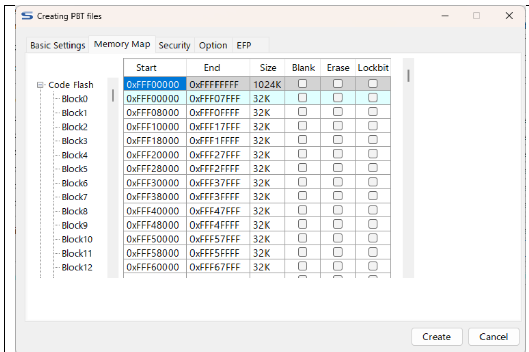
Figure 2.2 Memory Map Tab
